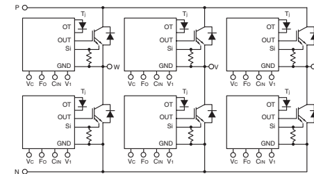
PM450CLA060, PM600CLA060
